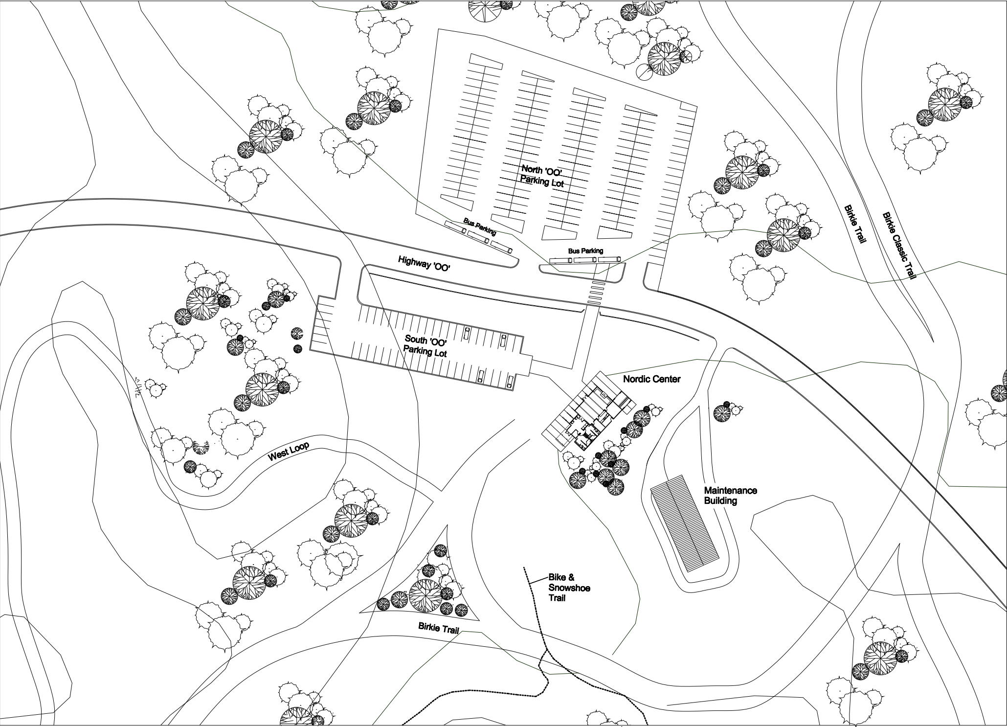
HIGHWAY 'OO' NORDIC CENTER SITE PLAN
